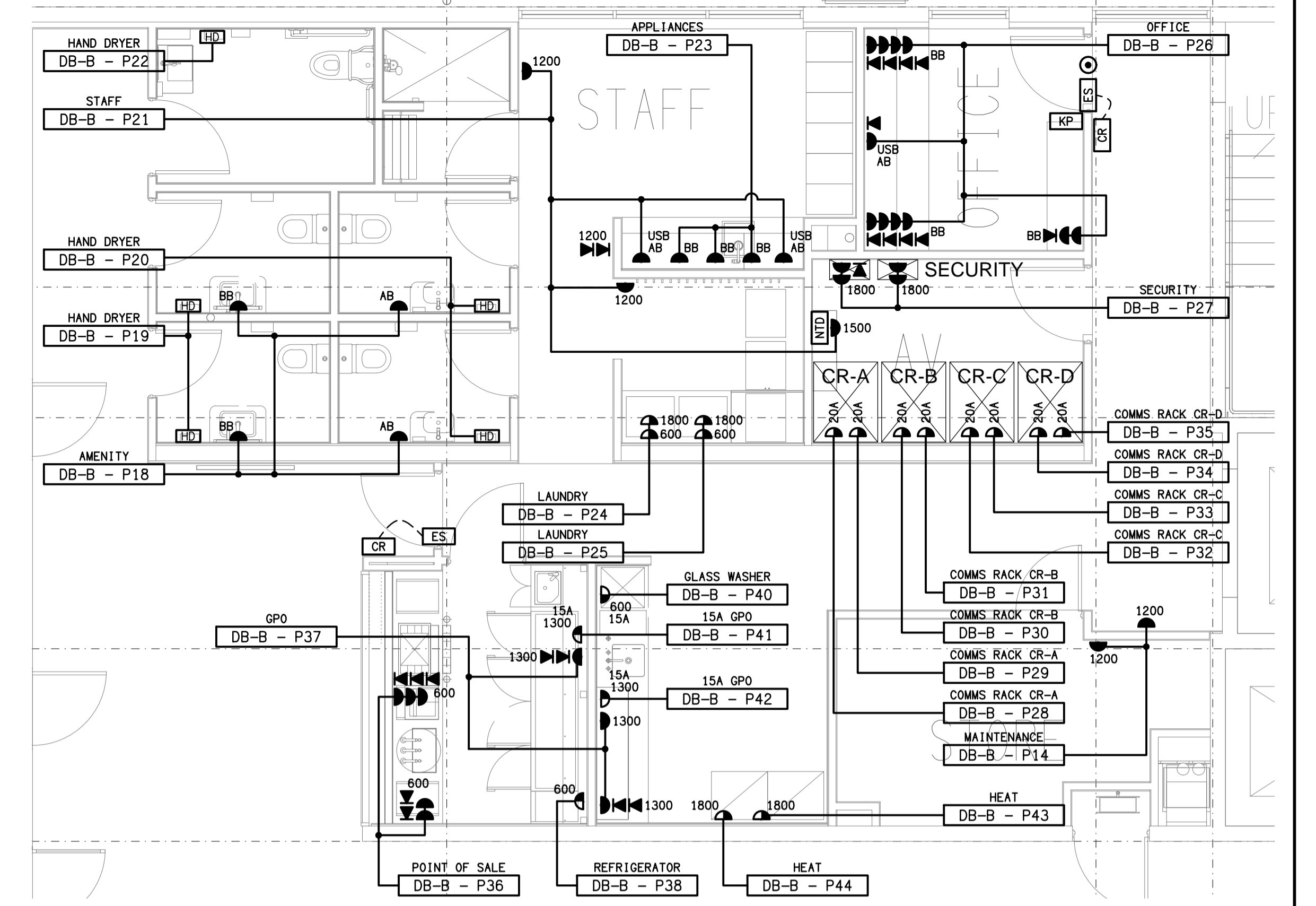
DETAIL A STAFF & BAR LAYOUT SCALE 1:50
